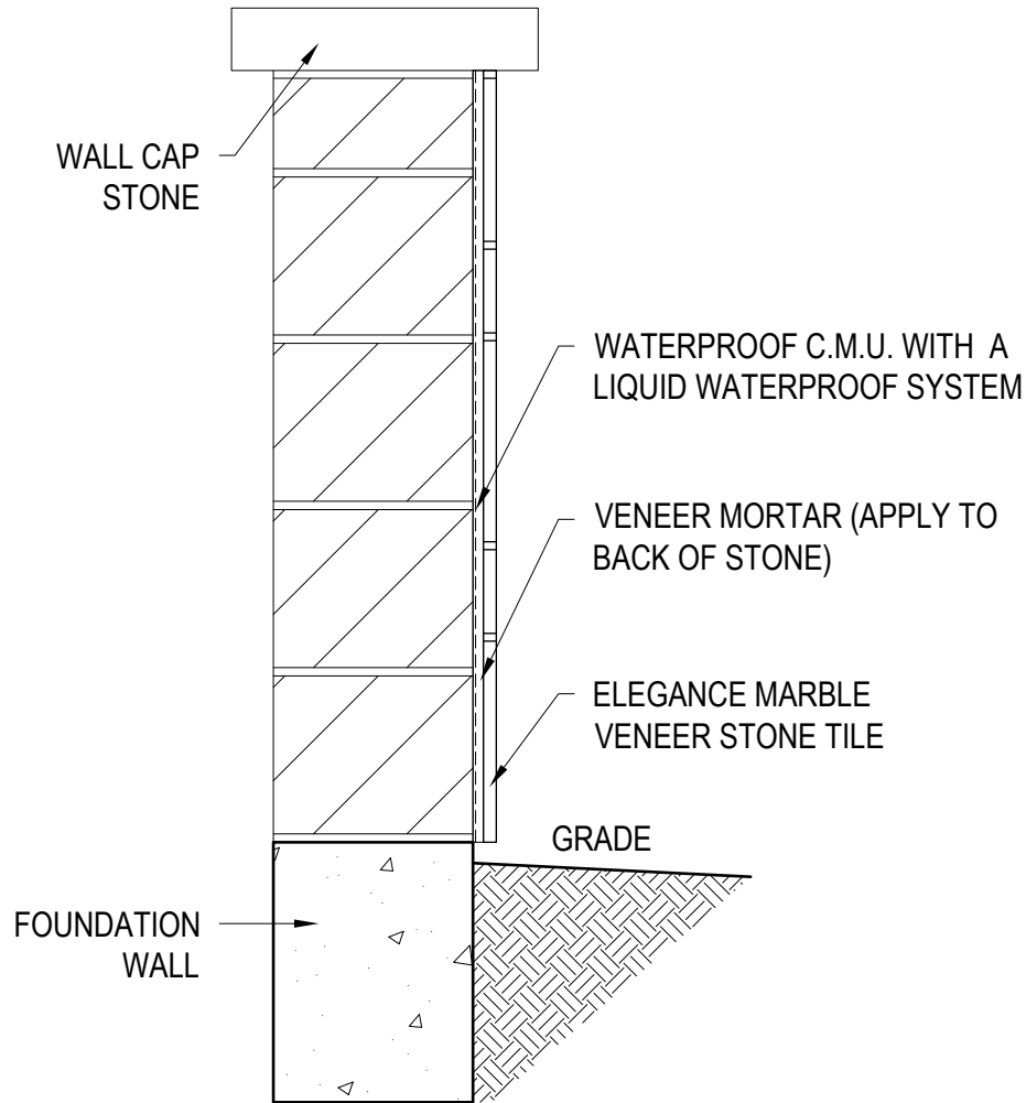
TYPICAL SECTION THIN VENEER INSTALLATION
