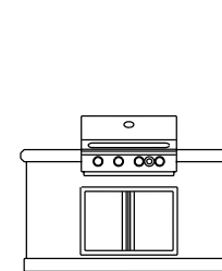
GRILL ISLAND 2'6" D X 5'11" W X 3'5" H (Grill and doors included)
