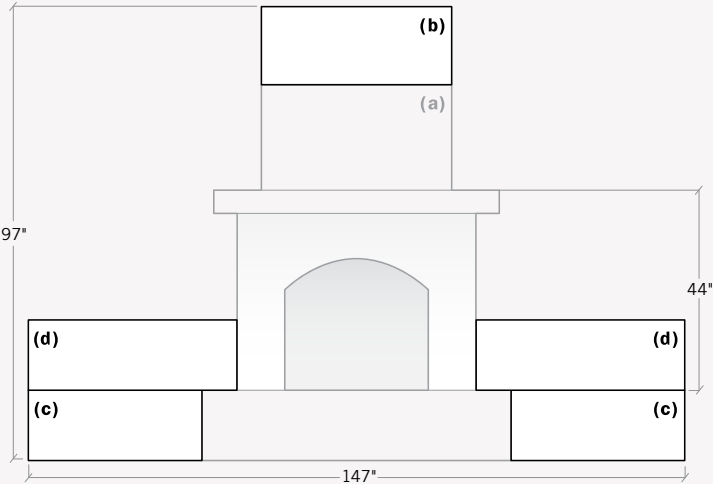
Gas-Burning Fireplace Extensions (a) Gas-Burning Fireplace | (b) Chimney Extension (c) Hearth Extension | (d) Hearth Extension Backrest
