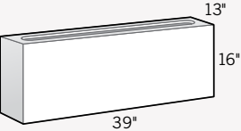
Wilmington Gas-Burning Fireplace Chimney Extension 13"D × 39"L × 16"H
