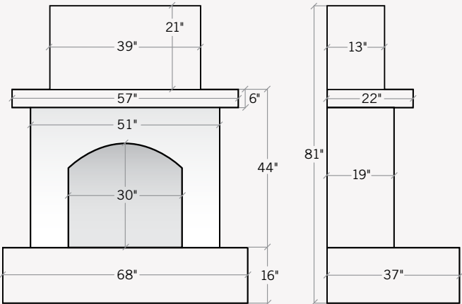
Wilmington Gas-Burning Fireplace 37"D × 68"L × 81"H
