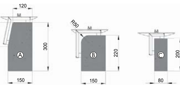
Quick Change device with integral suction plate for retrofitting for previous version
