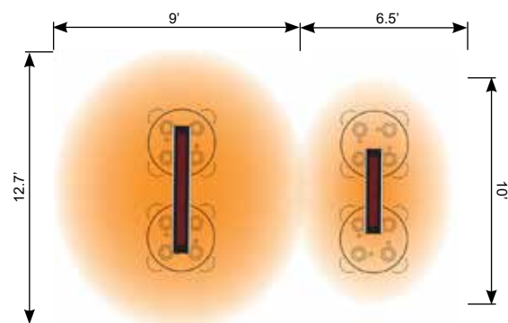
Ceiling Mounted Platinum w/ 48" Tube Suspension Kit
