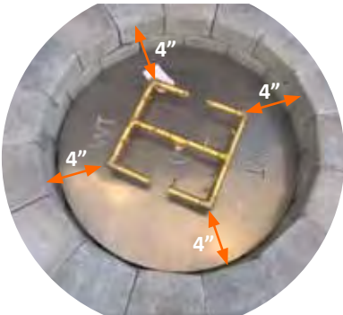
Recommended Burner Distance from Edge of Fire Pit
